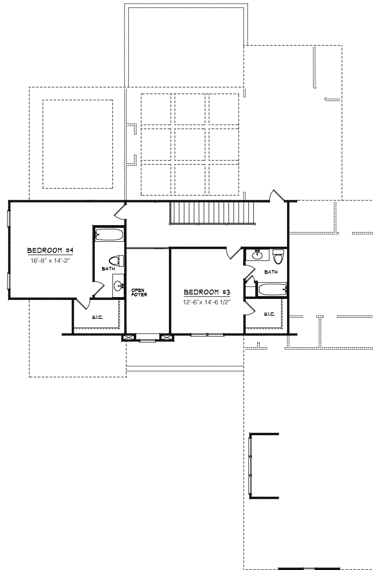
Second Level Plan 846 sq. ft. Heated 1596 sq. ft. Unheated
